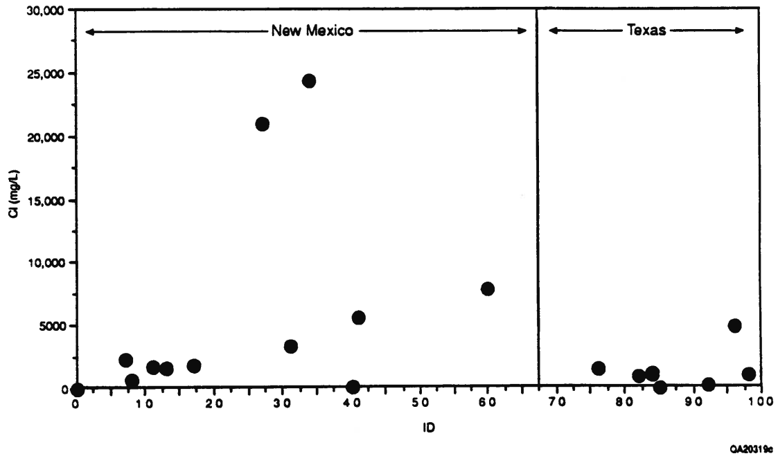
Figure 8. Chloride concentration in river-survey samples collected between Ute Reservoir, New Mexico, and Lake Meredith, Texas, February 1992.
