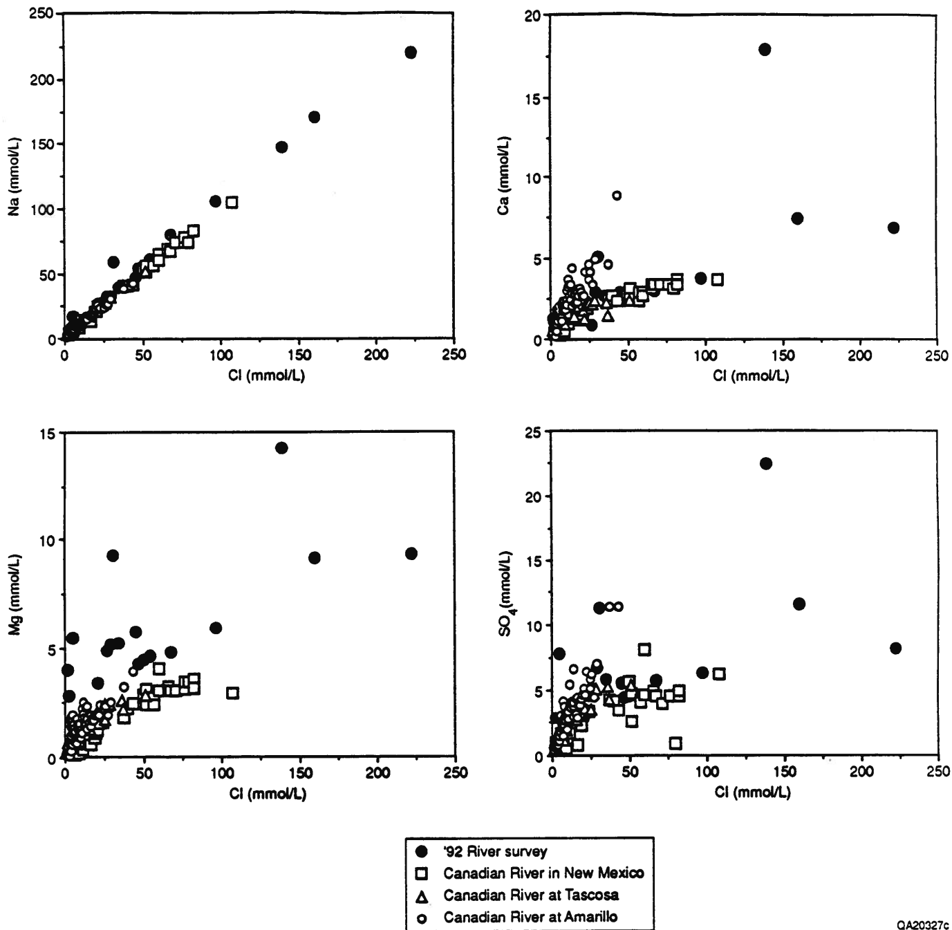
Figure 16. Comparison between February 1992 river-survey data (solid dots) and data from previous investigations in New Mexico (open squares), at Tascosa, Texas (open triangles) and at Amarillo, Texas (open circles) (previous data from Hydro Geo Chem, 1984).
