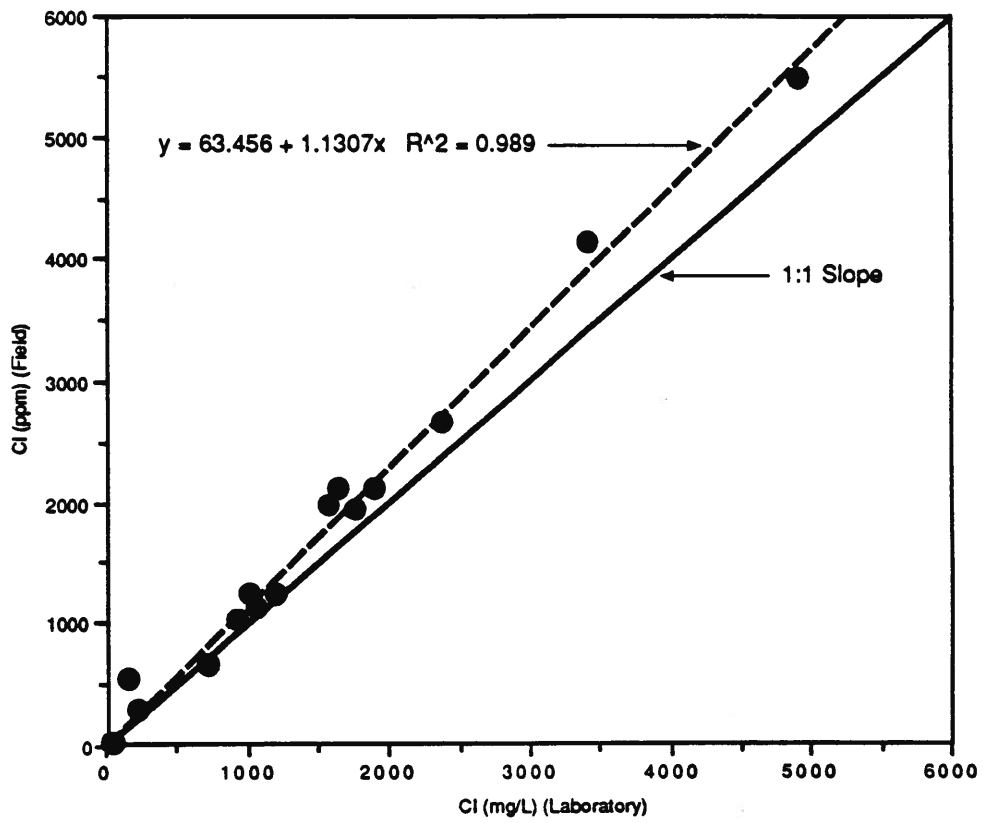
Figure 6. Comparison between chloride content determined in the field and chloride content determined in the laboratory for February 1992 river-survey samples.
