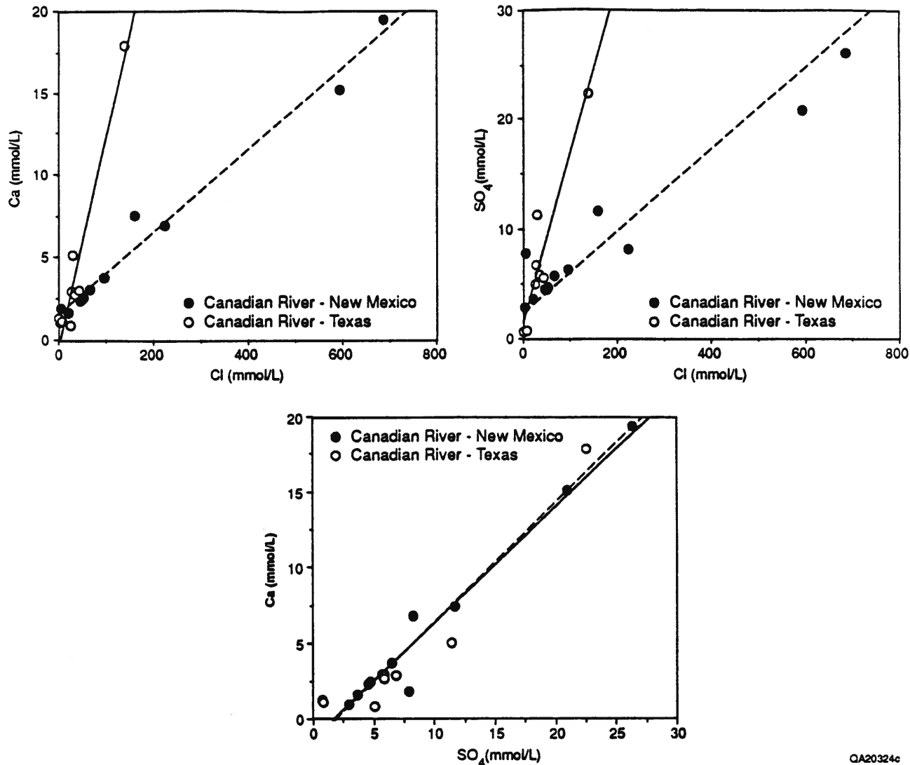
Figure 13. Bivariate plots of Ca, SO 4 , and Cl for river-survey samples. The plots differentiate between samples collected in New Mexico (solid dots) and those collected in Texas (open circles). Samples from the Texas reach typically exhibit larger Ca/Cl and SO 4 /Cl ratios than do samples from the New Mexico portion of the river.
