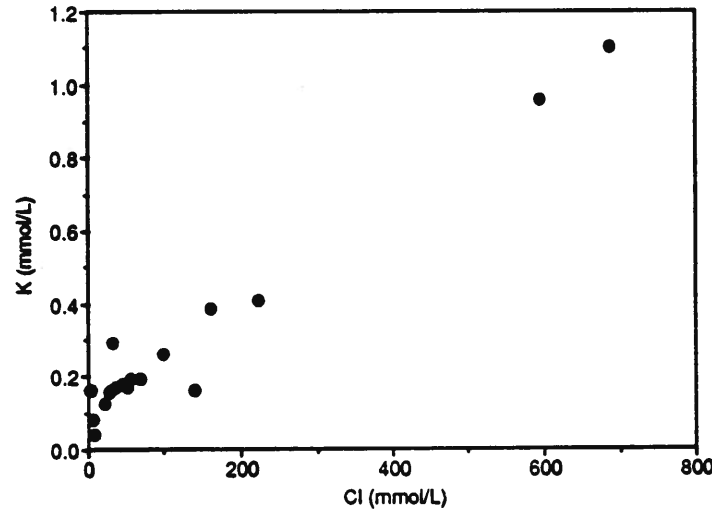
Figure 9. Bivariate plots of Ca, Mg, and K versus Cl for river-survey samples. The plots suggest mixing trends between low-Cl and high-Cl waters.
